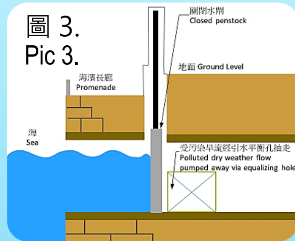
Penstocks are closed when HKO forecasts no rain in the coming 3 days. Seawater trapped inside the box culvert is pumped away.
